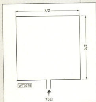
Fig. 3: Although not (strictly speaking) a derivation of the dipole, the loop antenna exhibits very similar properties to the basic dipole (see text).
