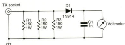
Fig. 1: Simple power reduction circuit (see text).
