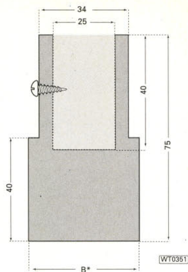
Fig. 4: The Nylon 66 joiner for the two lower sections of the antenna. Dimension B to be a tight fit inside the lower tube.
