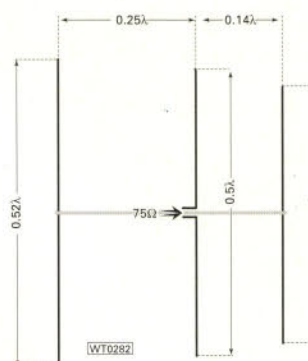
Fig. 6: The basic dipole antenna, used in conjunction with the familiar reflector and directors is known as the Yagi. The more elements used, the lower the feed impedance will become (see text).
