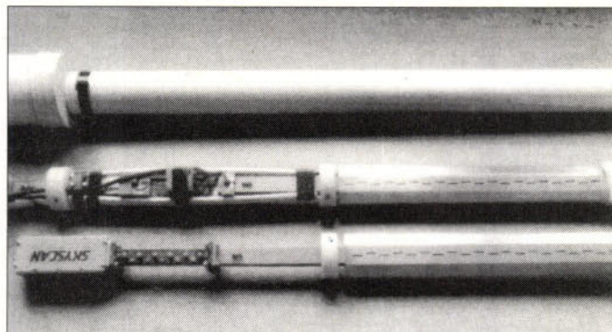
Microwave antennas aren't always dishes! There are 10GHz slotted waveguides, producing an all-round (omni-directional), horizontally polarised radiation pattern for the GB3XG Repeater.
