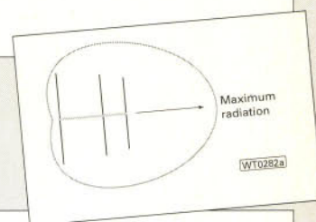
Fig. 6a: A three element Yagi and associated radiation pattern.
