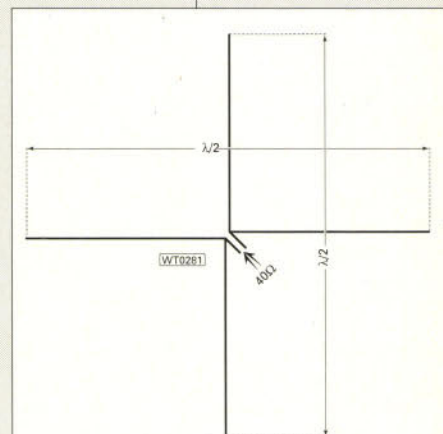
Fig. 5: Feeding multiple dipole antennas, although providing many advantages, also reduces the feed point impedance (see text).
