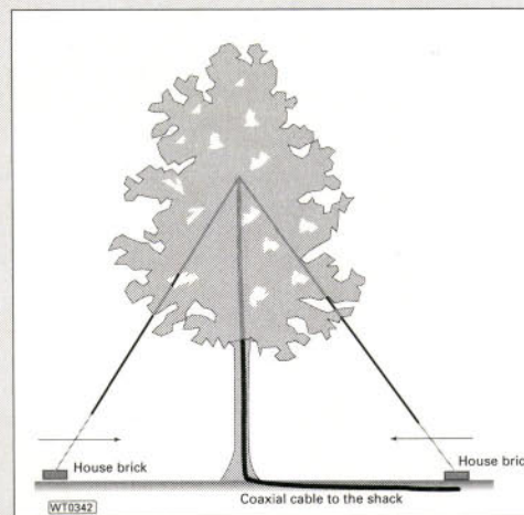
Fig. 3: Burying the centre of an inverted 'V' antenna in a tree doesn't seem to harm the signal much, as long as the ends are in the clear. The house bricks keep the antenna stretched but allow movement when the tree sways.
